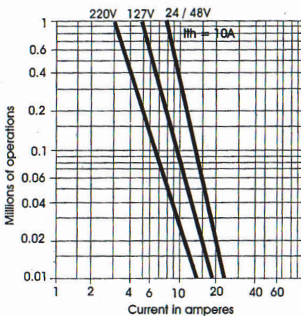
AC Ratings, Inductive - NEMA A600 35% Power Factor
